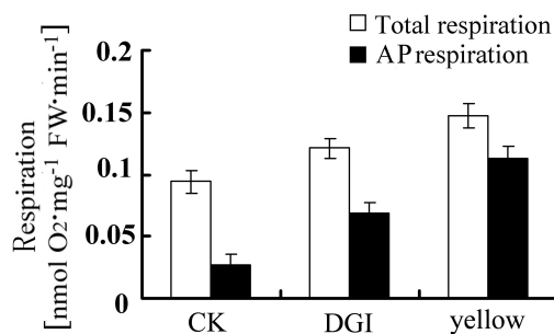
Fig. 4. Alternative pathway (AP) capacity and total respiration content of dark green island (DGI) and yellow leaf tissue (yellow) of CMV-infected Nicotiana tabacum leaves. Bars represent standard deviations of 3 independent replicates ( n = 3 ). CK, control.
