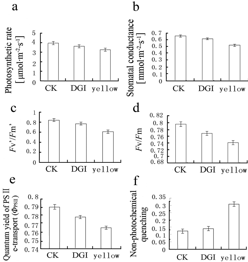
Fig. 5. Leaf net photosynthetic rate, stomatal conductance, Chl fluorescence parameters F_v'/F_m' , F_v/F_m , PSII quantum yield ( \Phi_{\text{PSII}} ), and non-photochemical quenching (NPO) of dark green island (DGI) and yellow leaf tissue (yellow) of CMV-infected Nicotiana tabacum leaves. Bars represent standard deviations of 3 independent replicates ( n = 3 ). CK, control.
